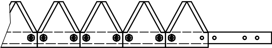
DETAIL C SCALE ( 1 : 4 )
